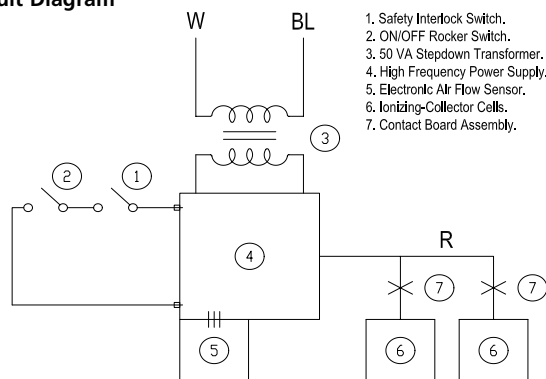
Circuit Diagram
