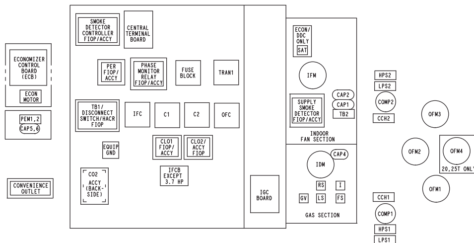
Fig. 4 Typical Power Diagram (2 Stage Cooling)
